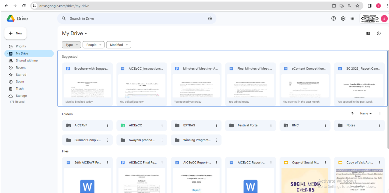
Image 3: Google Drive
