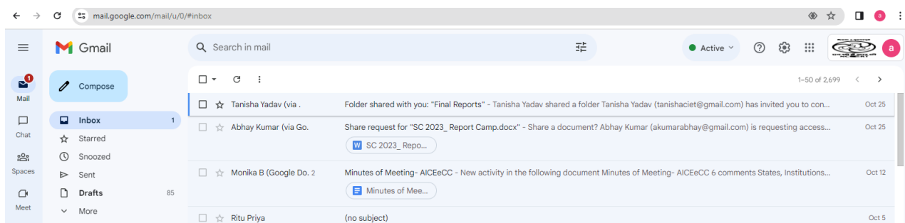
Image 1: Gmail account
